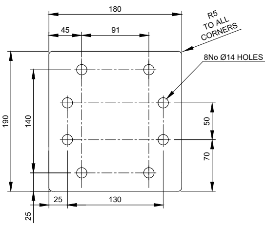
TPB-B-5 - 10mm THICK Scale 1:5
