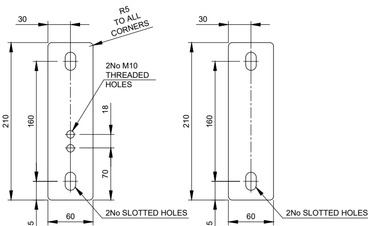
PART TPS-R-1 Scale 1:5
