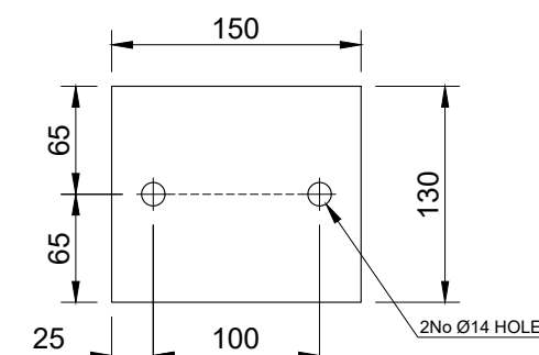
TPL-C-2 - 10mm THICK Scale 1:5
