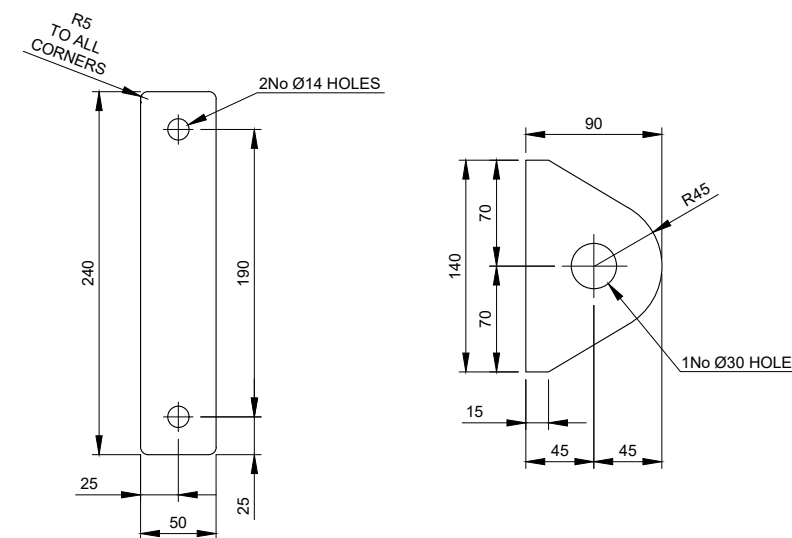
TPB-C-1 - 10mm THICK Scale 1:5
