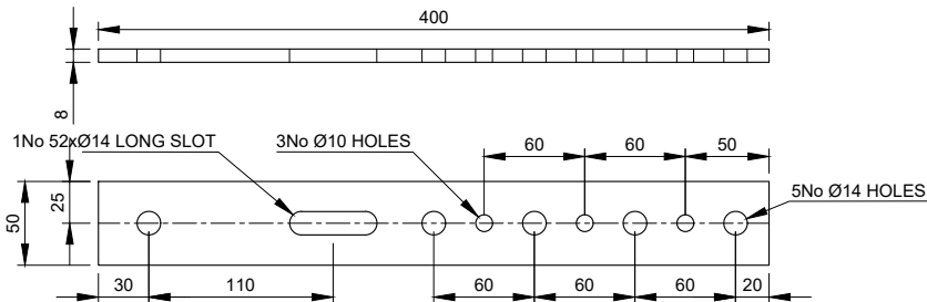
TPA-PD - 8mm THICK Scale 1:5
