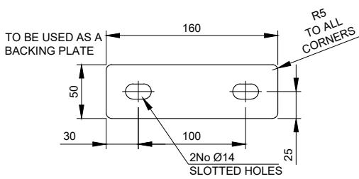
TPB-B-4 - 5mm THICK Scale 1:5
