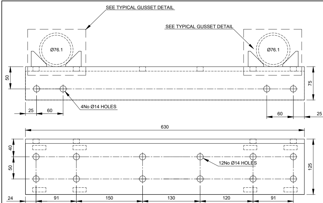
TPA-M - UA125x75x10 Scale 1:5
