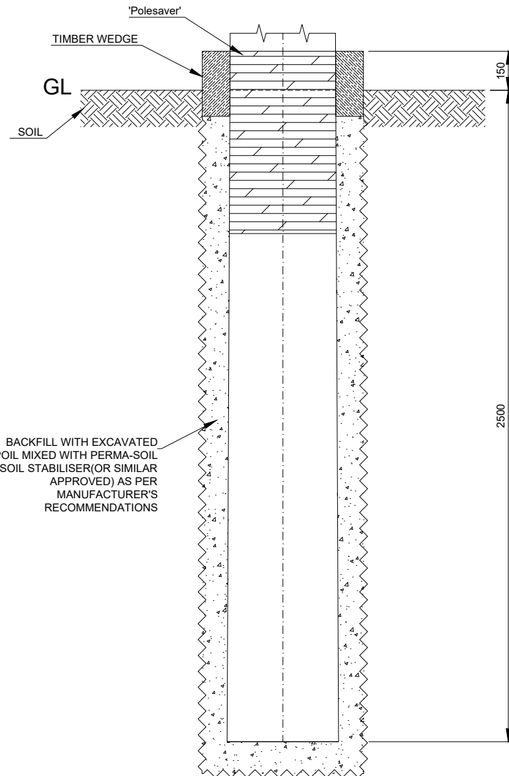
PORPOSED INSTALLATION ELEVATION Scale 1:20
