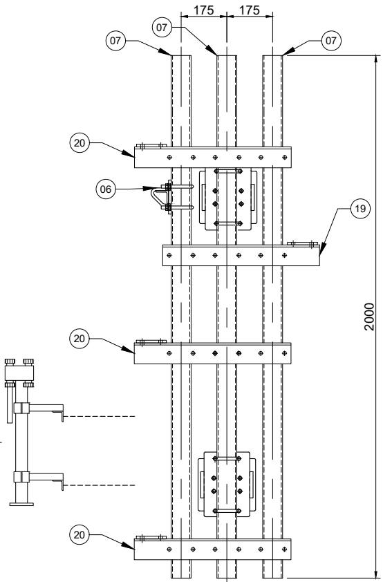
VIEW B-B Scale 1:20
