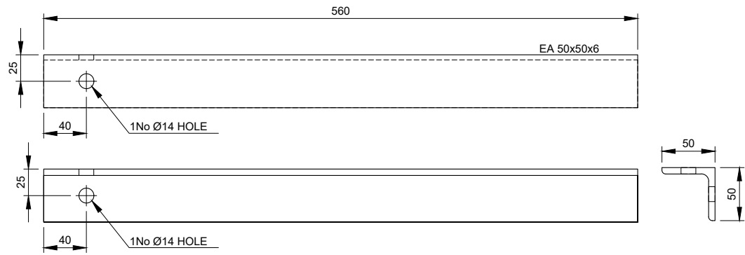
TPB-BR-1 - EA50x50x6 Scale 1:5
