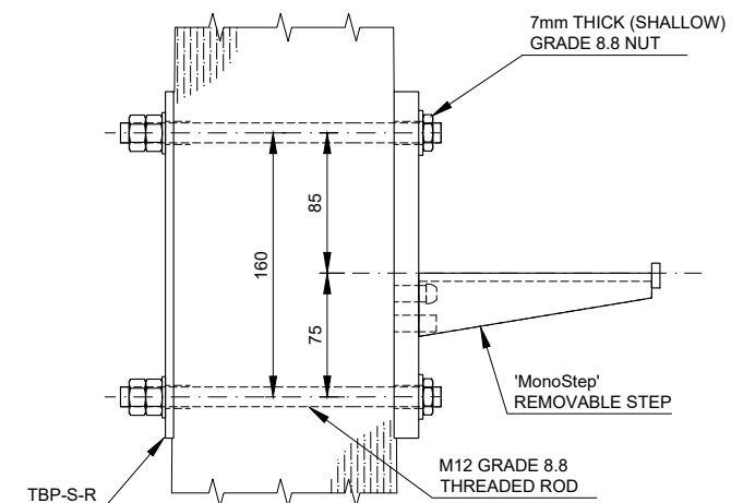
DETAIL F - REMOVABLE CLIMBING STEPS Scale 1:5
