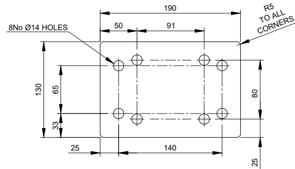
TPB-BR-3 - 10mm THICK Scale 1:5
