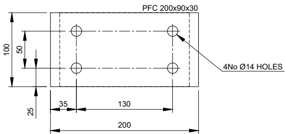
TPB-B-2 - PFC 200x90x30 Scale 1:5
