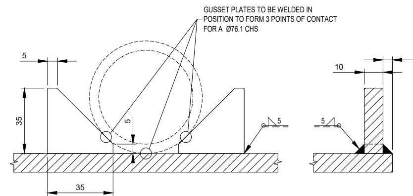
TYPICAL GUSSET PLATE DETAIL Scale 1:2
