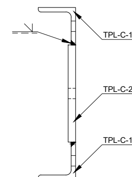
VIEW A-A Scale 1:5
