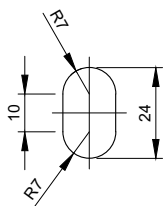
SLOTTED HOLE DETAIL Scale 1:2
