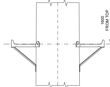
DETAIL D - ANTENNA ACCESS CLIMBING STEP Scale 1:10
