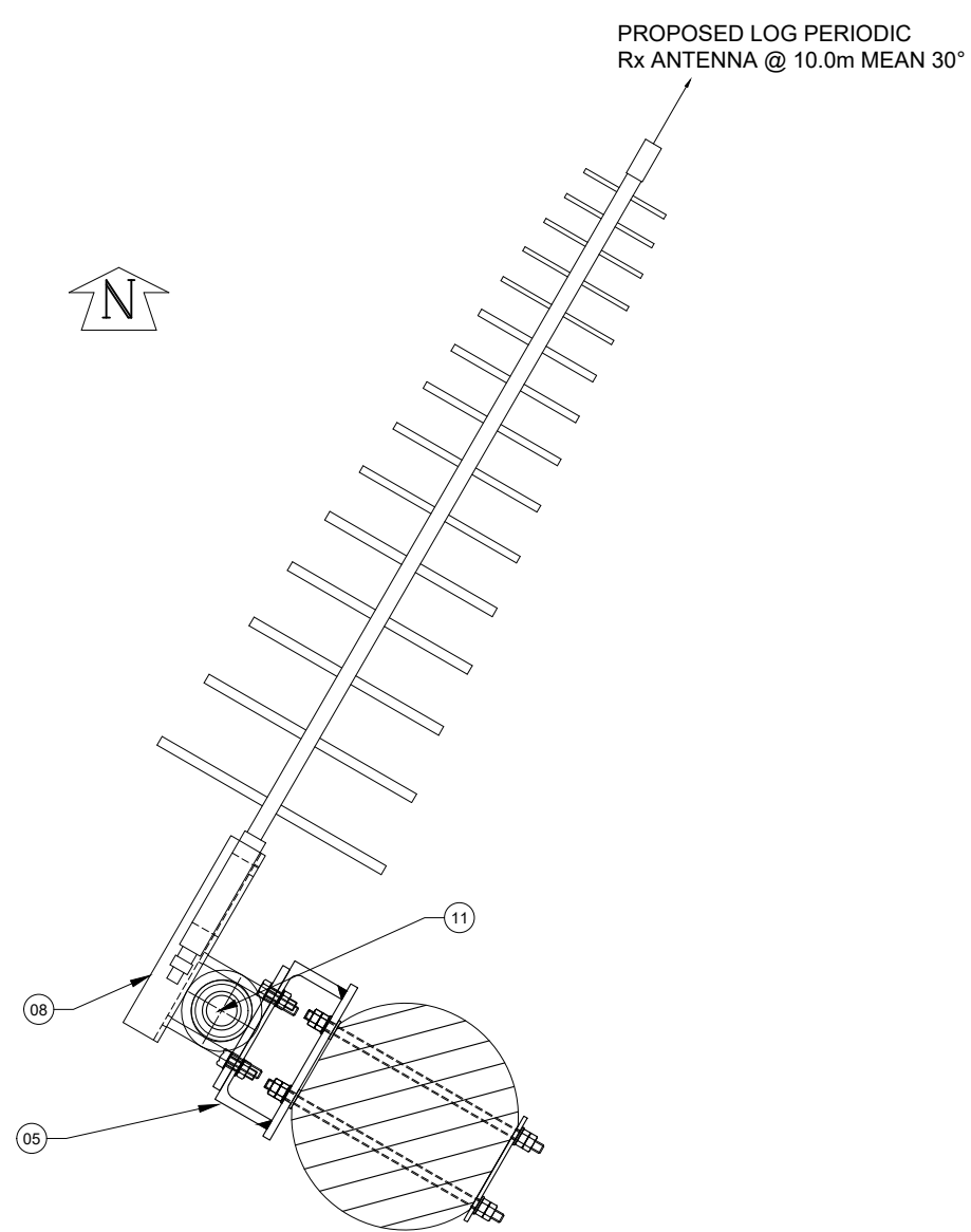
VIEW A-A Scale 1:10
