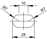
SLOTTED HOLE DETAIL Scale 1:2
