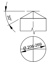
DETAIL A - TIMBER POLE TOP Scale 1:20
