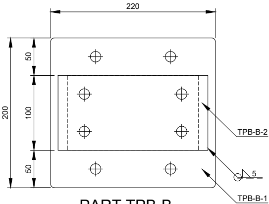
PART TPB-B Scale 1:5
