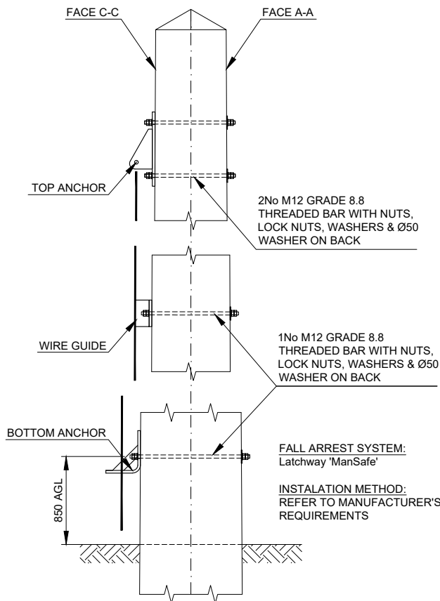
DETAIL B - FALL ARREST SYSTEM Scale 1:20
