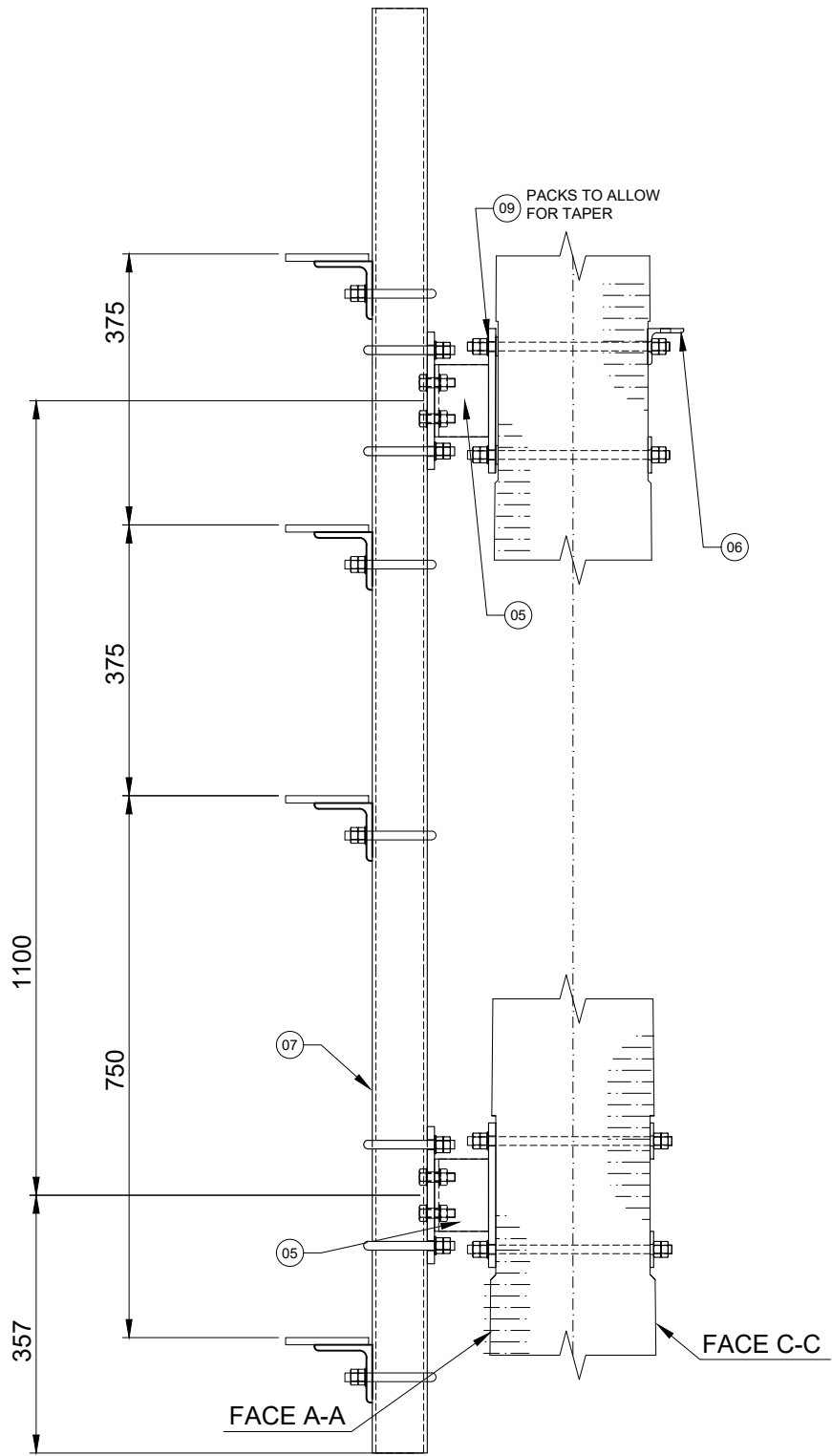
DETAIL G - Tx ANTENNA MOUNT Scale 1:10
