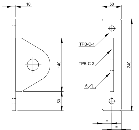
PART TPB-C Scale 1:5
