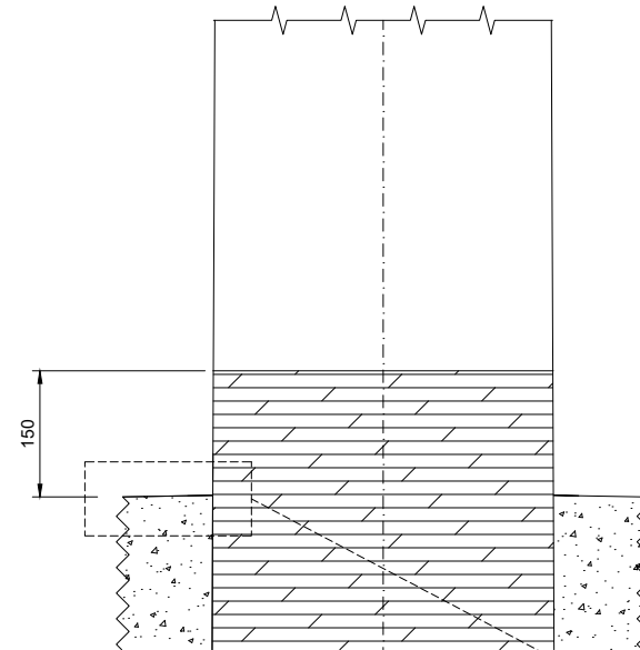
WATER PROOFING Scale 1:10
