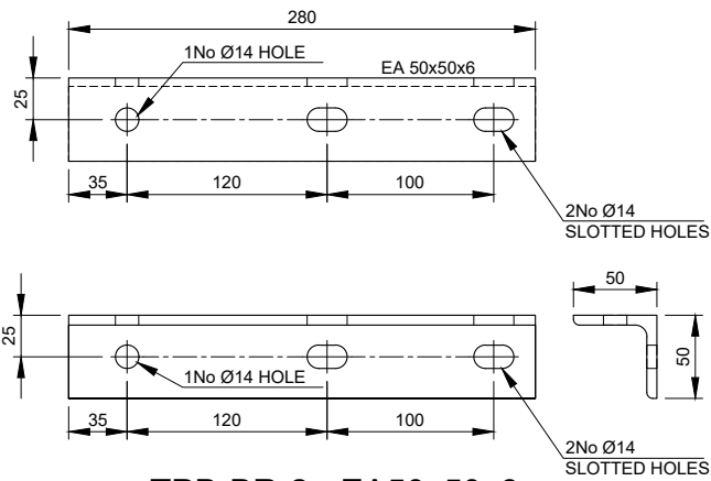
TPB-BR-2 - EA50x50x6 Scale 1:5
